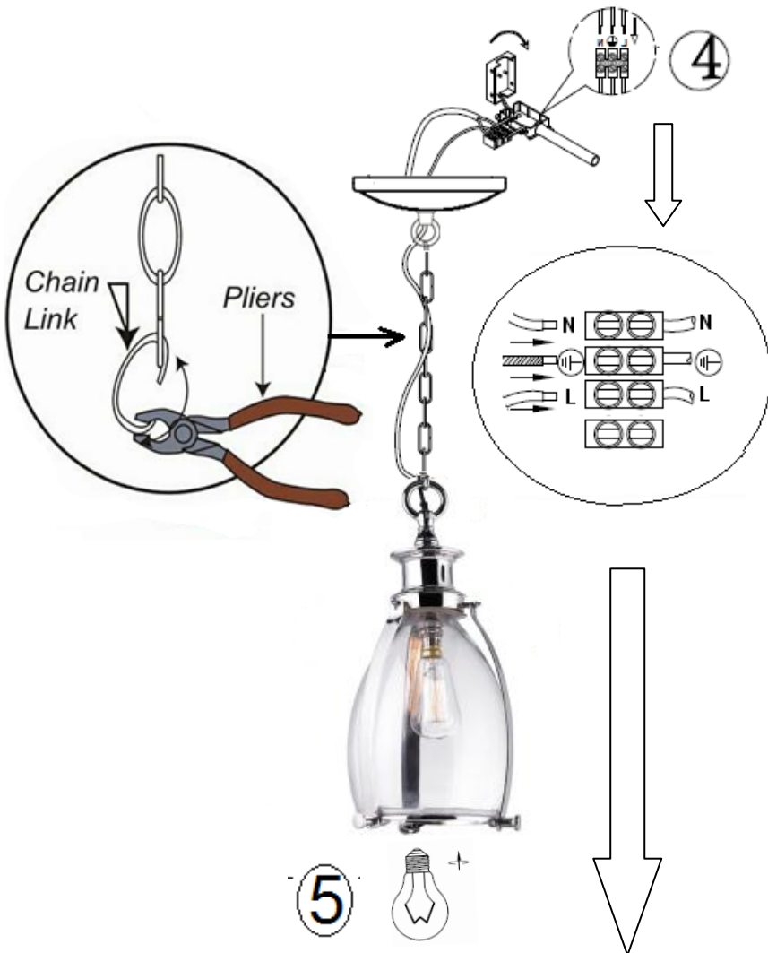
Wiring Details
