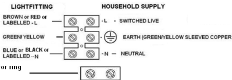
Wiring Details
